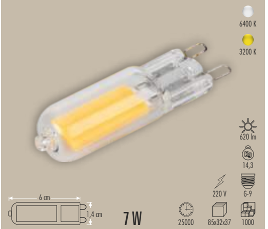
CT-4222 COB LEDLİ G-9 KAPSÜL 220 V
